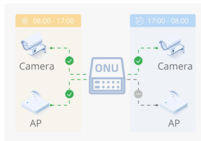
PoE Scheduling
